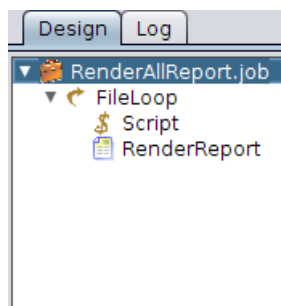
Figure 5.1. FileLoop Tree
