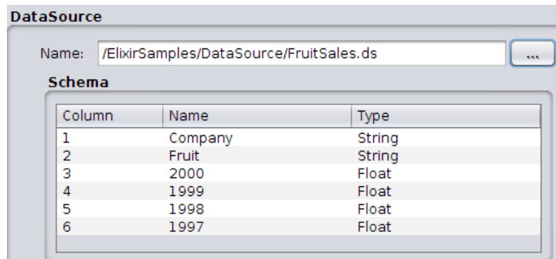
Figure 2.4. DataLoop
